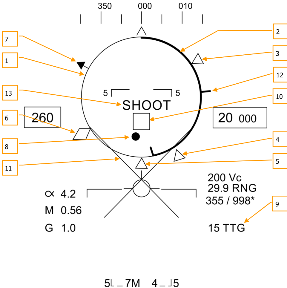
Figure 82. AIM-7 HUD with L&S Target
