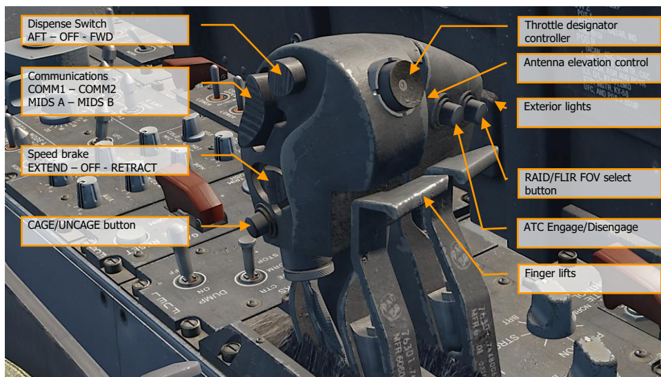
Figure 18. Throttles
