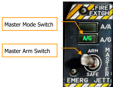
Figure 50. A/G Master Mode Select
