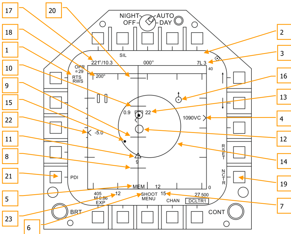
Figure 83. AIM-7 RADAR with L&S Target
