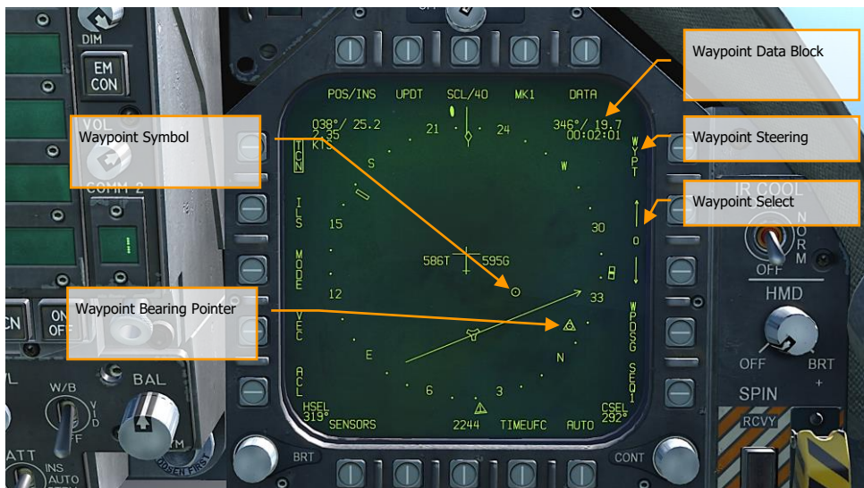
Figure 38. HSI Waypoint Steering
