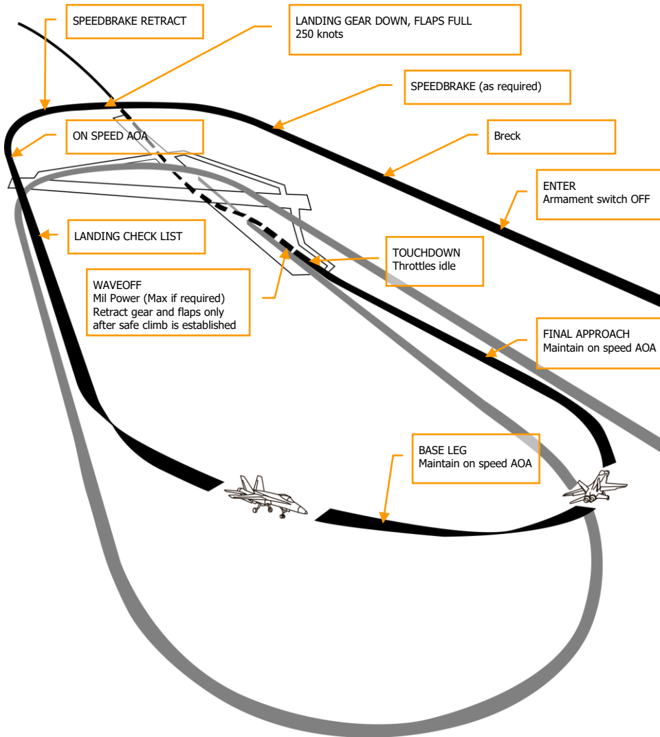
Figure 33. Airfield Landing Pattern
