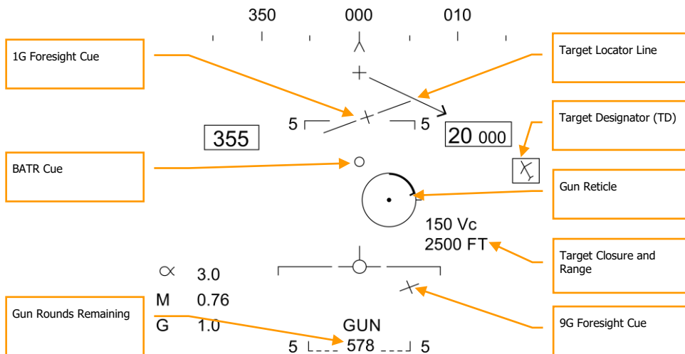
Figure 72. A/A GUNS HUD, Radar Tracking Mode
