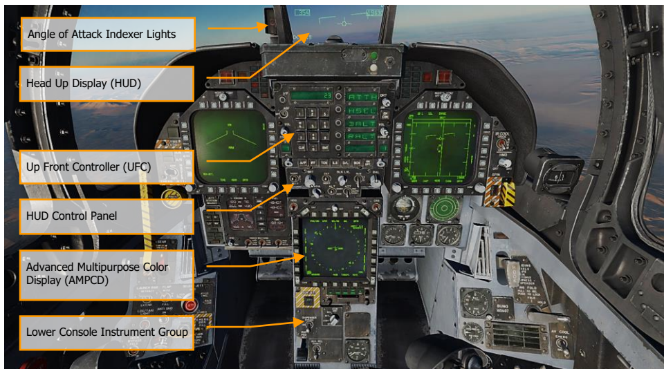
Figure 10. Center Instrument Panel
