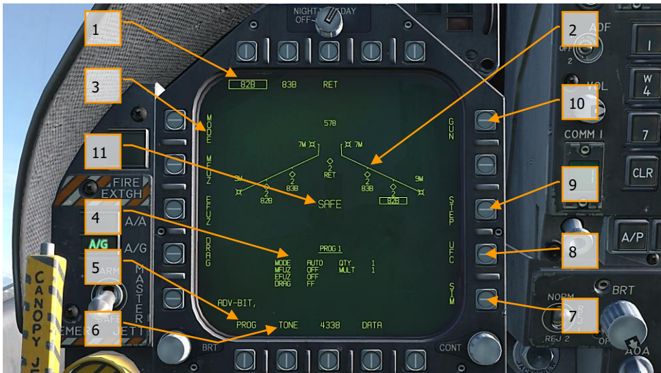
Figure 51. A/G Conventional Bombing SMS Page
