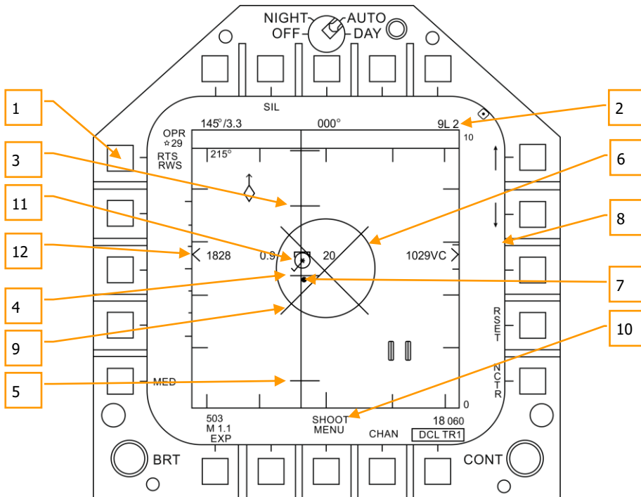
Figure 77. AIM-9 RADAR, RADAR Locked Target
